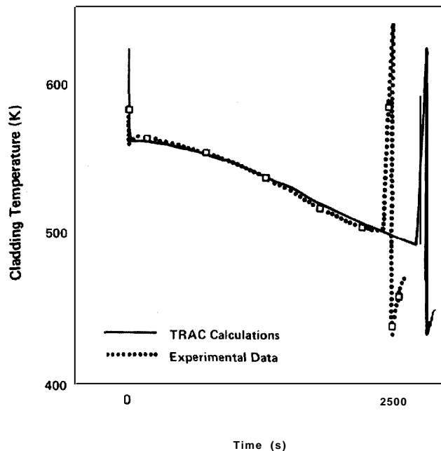
Fig. 17. Cladding temperatures during a simulated small-break loss-of-coolant accident at LOFT with the primary pumps operating until about 2400 seconds.
